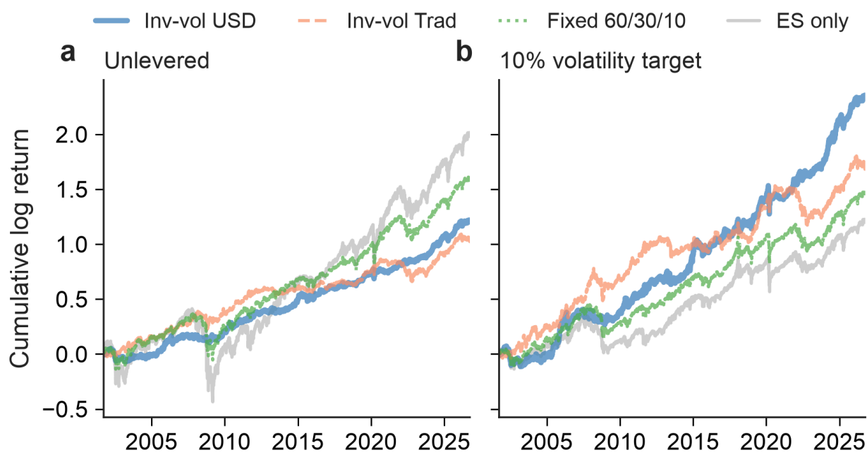
Figure 16: Futures portfolios on their common window (2001-10-01 → 2026-10-02). a , unlevered cumulative log returns. b , the same books scaled ex ante to a 10% volatility target at every rebalance (Section 8.5). Grey = ES alone.
