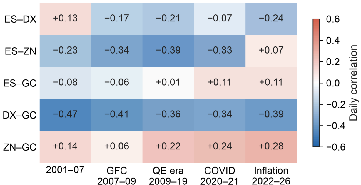
Figure 8: Daily correlation by regime for every asset pair in the two baskets (blue = diversifying, red = moving together).
