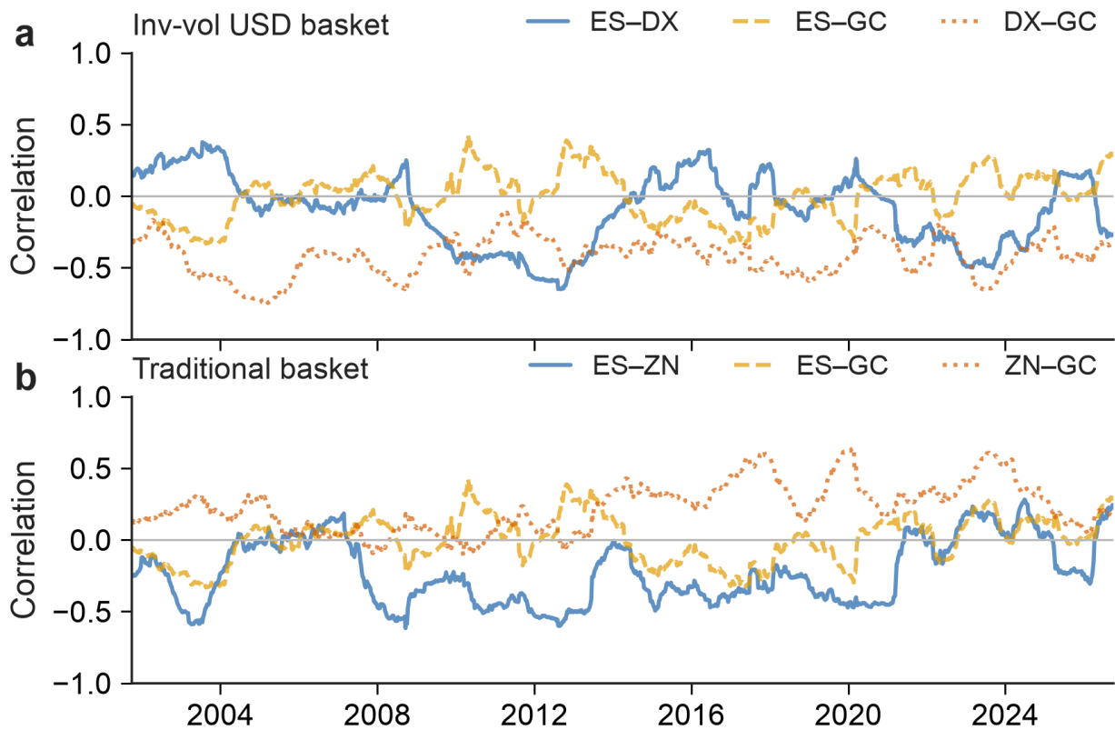
Figure 7: 252-day rolling pairwise correlations of daily log returns. a , assets of the Inv-vol USD basket. b , assets of the traditional basket. ES–GC appears in both panels.
