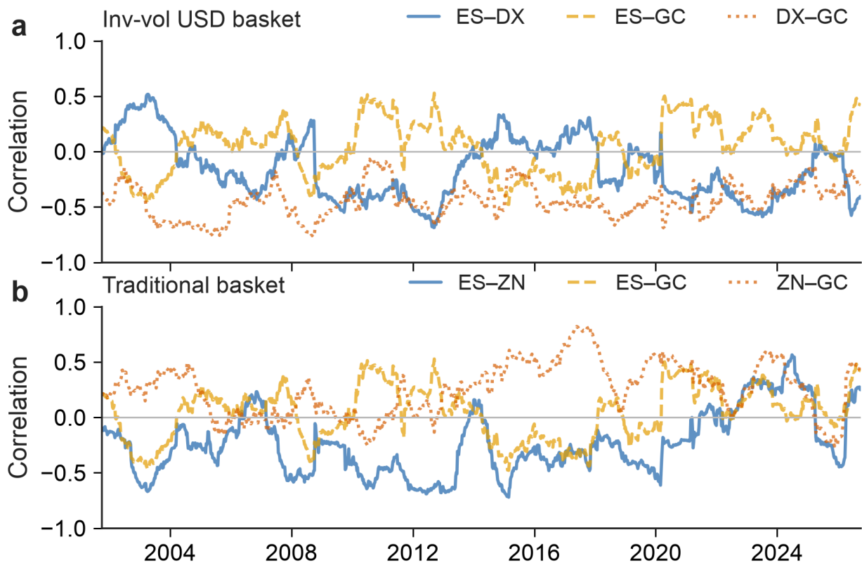
Figure 7: 52-week rolling pairwise correlations of weekly log returns (the futures settle at different times of day, which dilutes daily correlations). a , assets of the Inv-vol USD basket. b , assets of the traditional basket. ES-GC appears in both panels.
