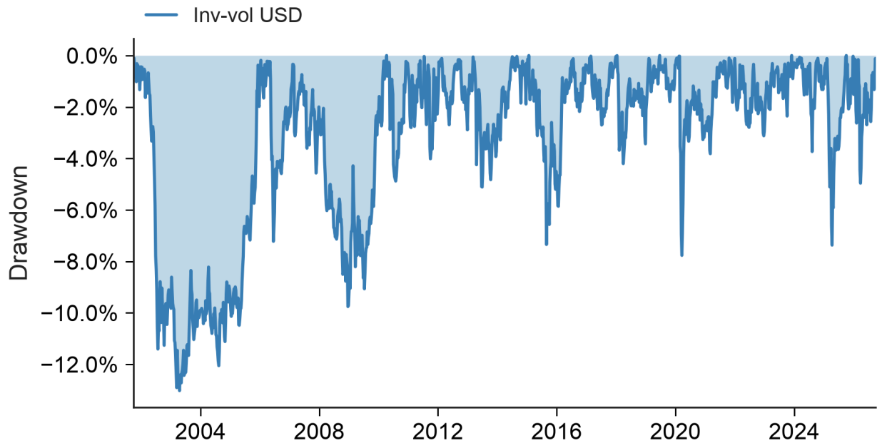
Figure 5: Ongoing drawdown of the unscaled inverse-vol USD futures portfolio.
