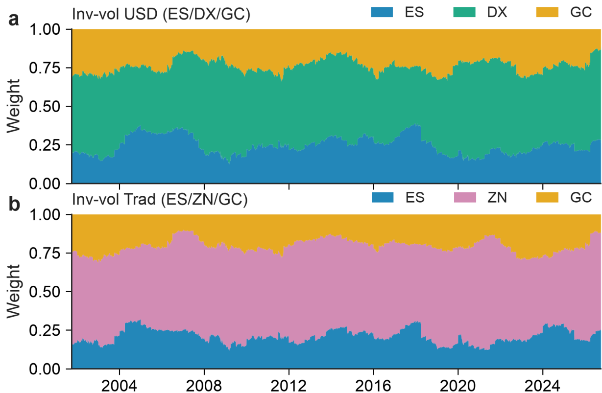
Figure 6: Actual daily weights with quarterly rebalancing (targets reset at each quarter-end, then drift). a , Inv-vol USD. b , Inv-vol Trad.
