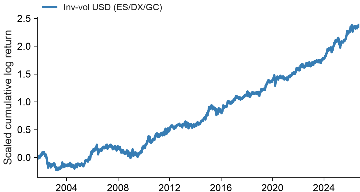
Figure 4: Inverse-vol USD futures portfolio (quarterly, drifting weights, after costs): cumulative log returns scaled to a 10% average annual endpoint for visual comparison of path shape.
