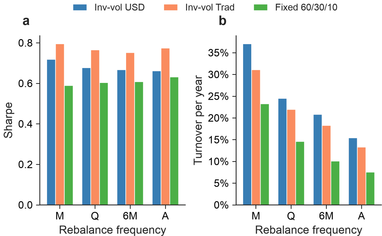
Figure 20: Effect of rebalance frequency (M = monthly, Q = quarterly, 6M = semi-annual, A = annual) on futures portfolios over a common window. a , Sharpe. b , annual turnover (sum of |\Delta w| ).
