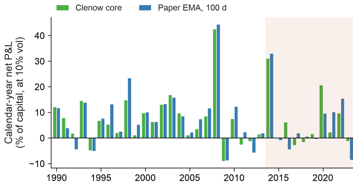
Figure 15: Calendar-year net P&L at 10% volatility, 1990–2023.
