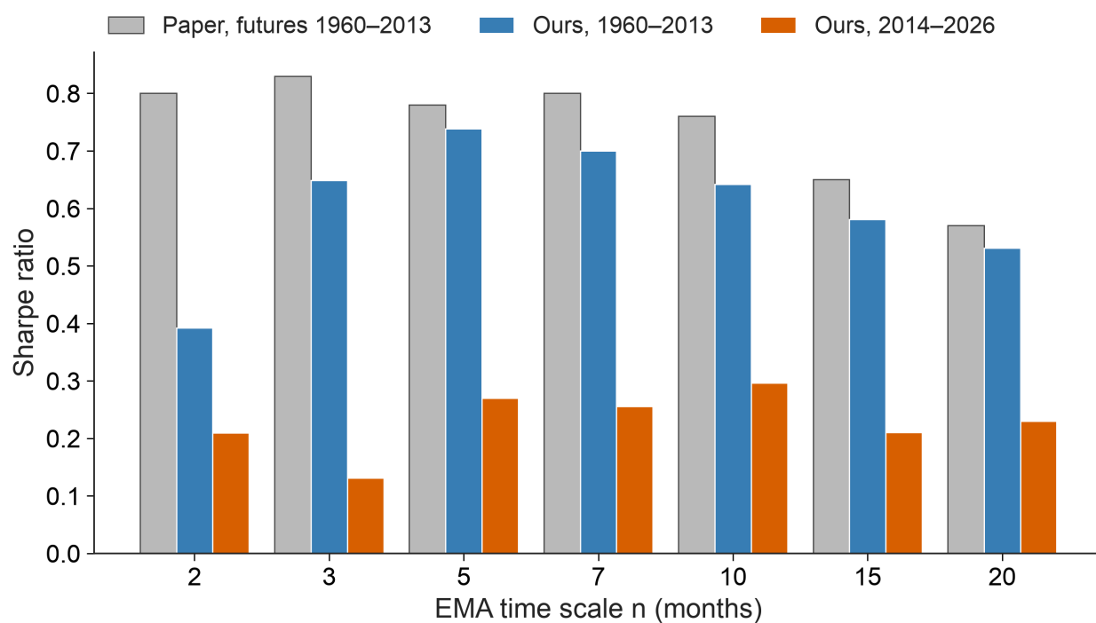
Figure 3: Sharpe ratio by EMA time scale: paper (futures), replication (spot proxies), and after publication.
