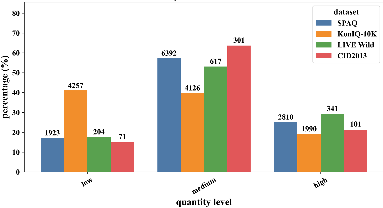
Quantity Level Distribution
