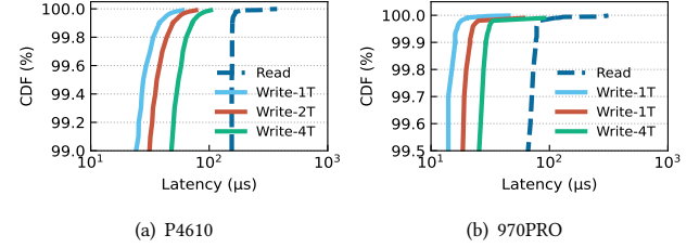
Figure 4: Effect of SSD internal buffer on write latency
