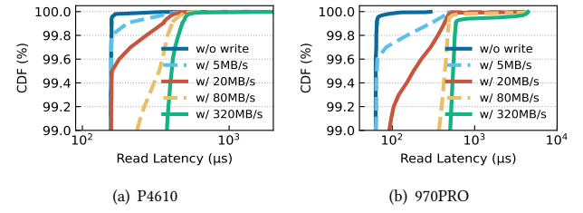
Figure 3: Impact of garbage collection on read latency
