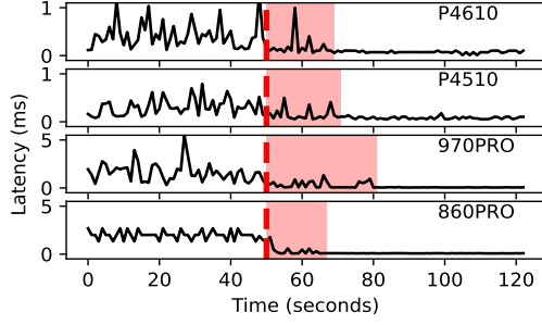
Figure 5: Impact of buffer flush on read latency
