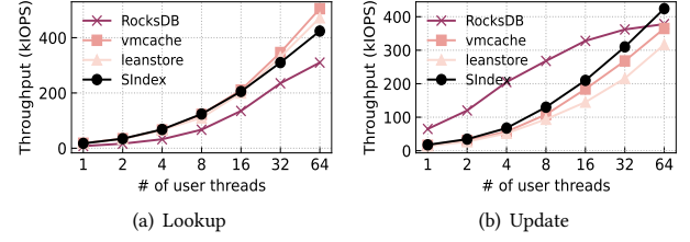
Figure 16: Throughput on different indexes
