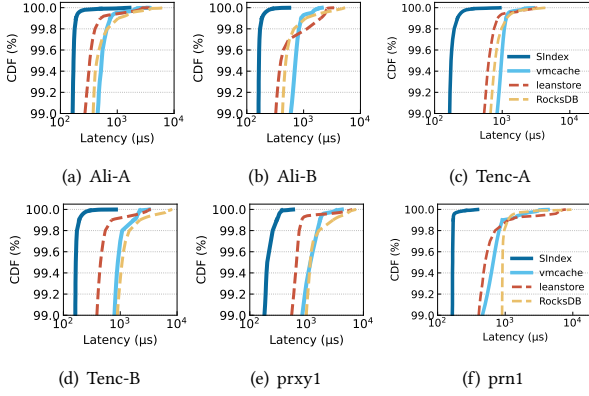
Figure 18: Latency CDF on trace-driven workloads
