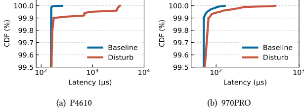
Figure 6: SSD Performance under read disturbance
