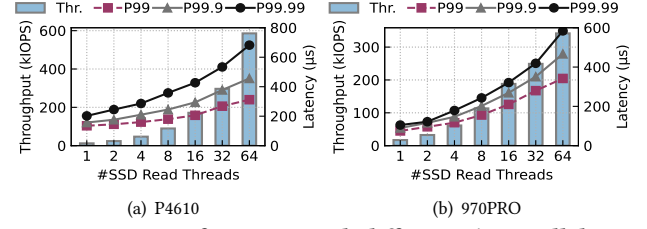
Figure 7: SSD performance with different I/O parallelism
