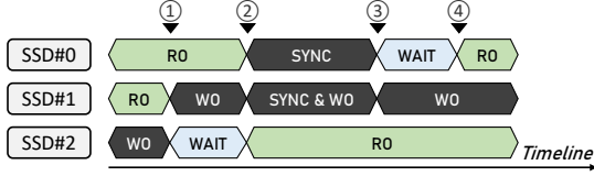
Figure 13: Workflow of state transition
