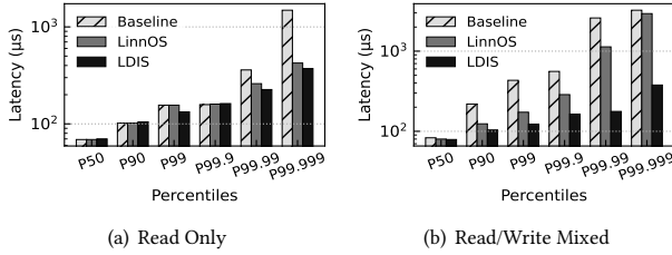
Figure 19: Latency of LDIS and LinnOS
