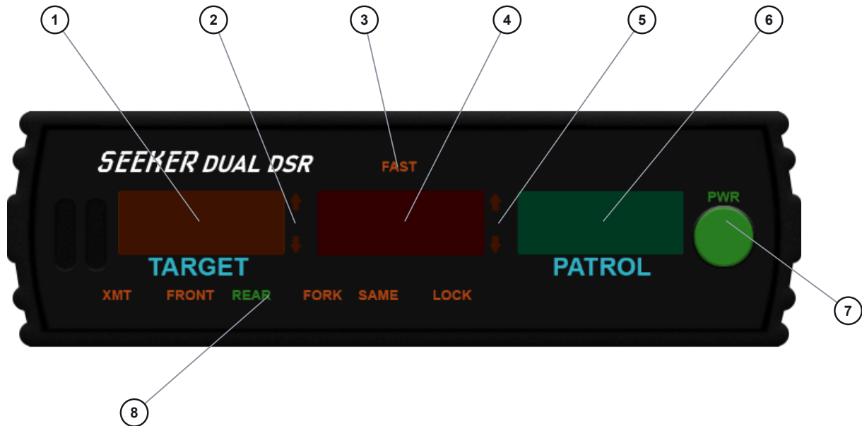
The display unit and its callouts.
