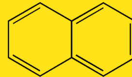
Naphthalene
