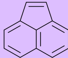
Acenaphthylene
