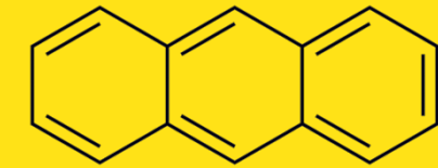
Anthracene
