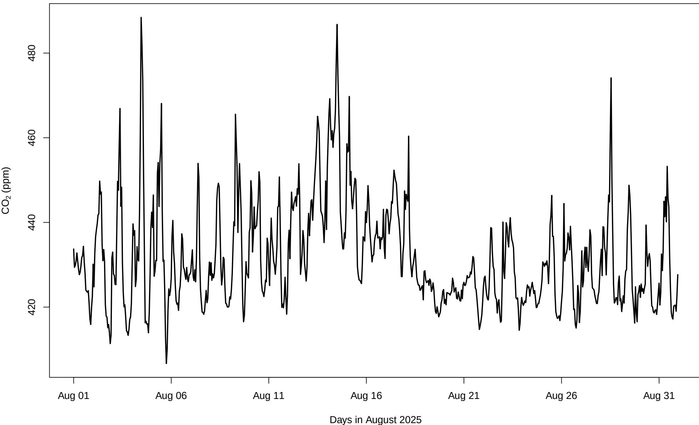
Sample Data: CO 2 Concentration at Columbia University (ASRC) Site – August 2025
