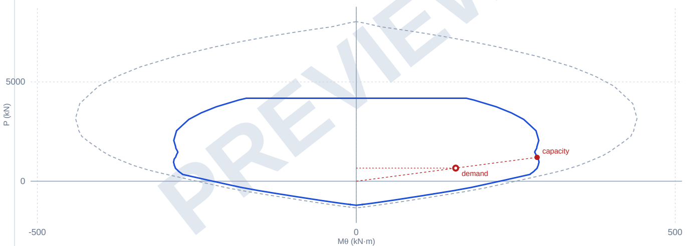
P-M \theta at \theta_L = 51.25^\circ , with the load point
