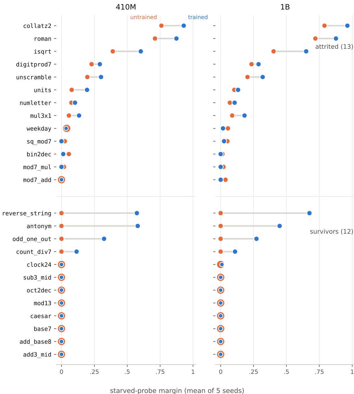
Figure 2: Trained versus untrained starved-probe margins per capability (means of 5 seeds), both model sizes; attracted capabilities above the divider, survivors below. An orange ring behind a blue dot marks coincident values. Survivors’ untrained margins are exactly zero in every cell; four survivors show trained structure the random network lacks entirely; and the top of the attracted block shows training adding structure on top of a leak, the rescuability signature described in the text.
