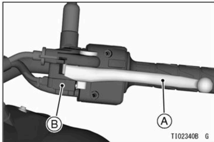
A. Clutch Lever B. Starter Lockout Switch
