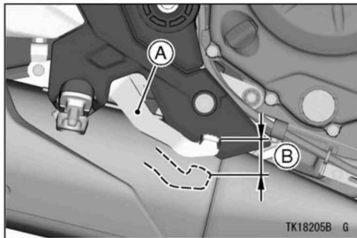
A. Brake Pedal B. 10 mm (0.39 in.)
