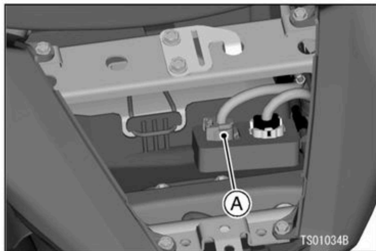
A. DFI System Diagnostic Connector
