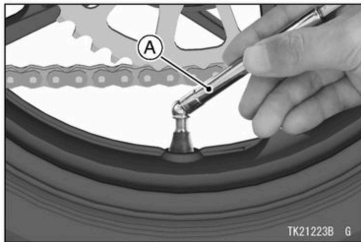
A. Tire Pressure Gauge
