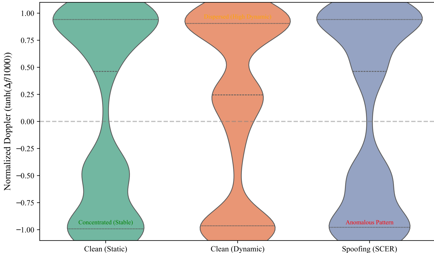
Feature Distribution after Physics-Aware Normalization
