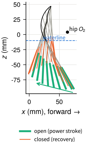
(a) Drag-type paddle, V3trap
