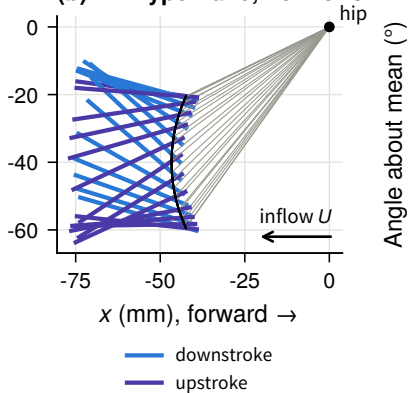
(b) Lift-type fluke, L0 motion
