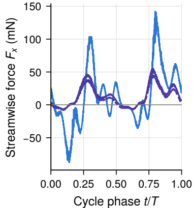
(c) Thrust history (smoothed)
