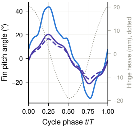
(a) Prescribed fin pitch
