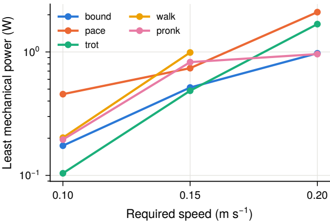
Gait families with lift, limits 10/5/5°
