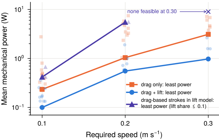
Drag vs. lift, limits 10/10/15°
