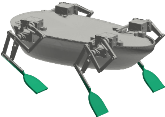
(a) Drag-type configuration (fan paddles)
