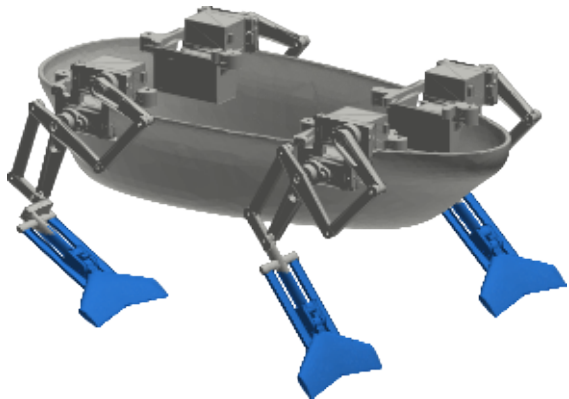
(b) Lift-type configuration (flukes)
