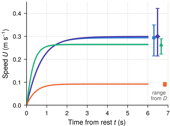
(b) Quasi-steady surge from rest
