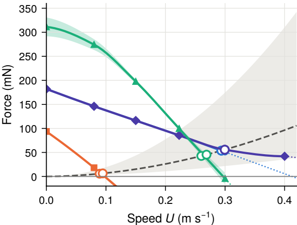
(a) Four-leg thrust 4\bar{T}(U) vs. resistance
