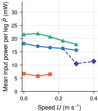
(b) Power
