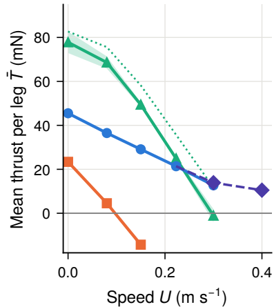
(a) Thrust
