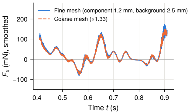
(c) Mesh sensitivity, window 0.41–0.91 s
