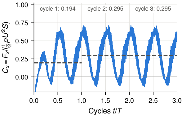
(c) Mesh sensitivity, window 0.41–0.91 s
