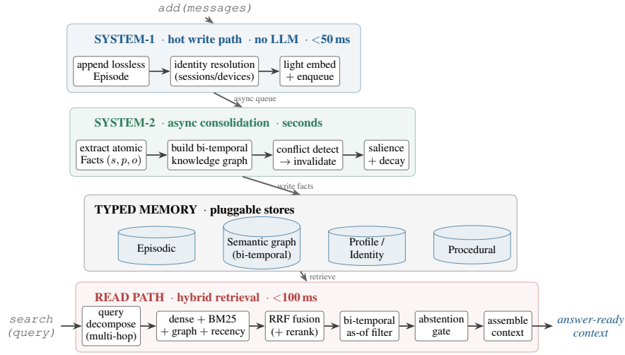
Figure 1: The ENGRAM dual-process architecture: a hot write path (SYSTEM-1) that never blocks on an LLM; an asynchronous consolidation path (SYSTEM-2) that extracts facts, builds the bi-temporal graph and resolves conflicts non-destructively; a typed memory over pluggable stores; and a hybrid read path (dense + lexical + graph + recency, fused by RRF) with an as-of filter and an abstention gate.
