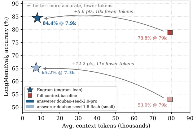
Figure 3: Accuracy vs. average context tokens on LongMemEval s (500 questions) for two answerer backbones: engram_lean (star) sits up and to the left of full-context (square)—+5.6 points at 10× fewer tokens for doubao-seed-2.0-pro, +12.2 at 11× for the small doubao-seed-1.6-flash (Table 3).
