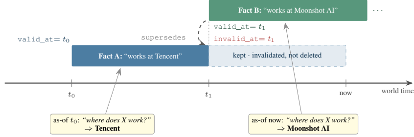
Figure 2: Bi-temporal facts make contradictions and “as-of” queries first-class: when Fact B arrives at t_1 , ENGRAM sets A.\text{invalid\_at} = t_1 and B.\text{supersedes} = A —A is invalidated, not deleted , so history and provenance survive—and a point-in-time query resolves against the fact valid at that time, which is what the knowledge-update and temporal categories require.
