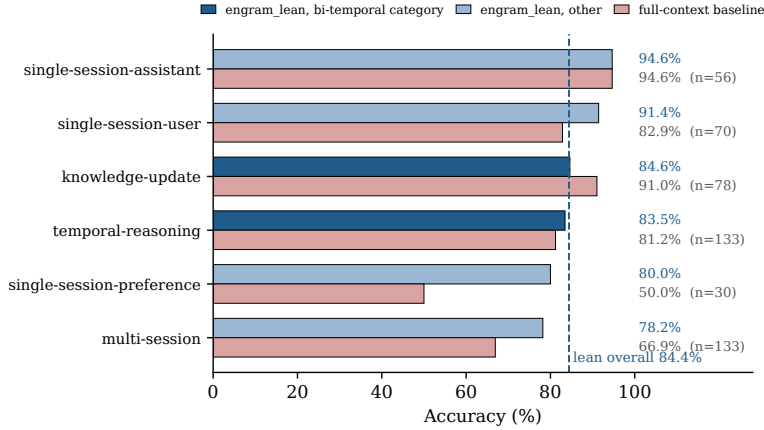
Figure 4: Per-category accuracy of engram_lean vs. full-context on the full 500-question set (dashed line: the 84.4% lean overall). The two bi-temporal categories are highlighted: temporal-reasoning a small win, knowledge-update the one loss; the largest margins are single-session-preference and multi-session.
