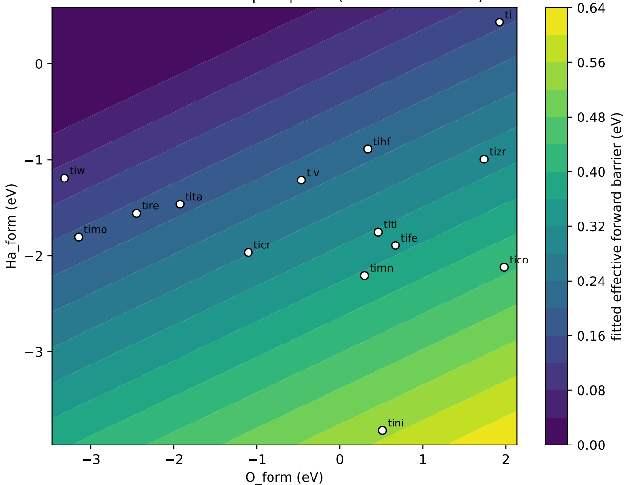
Linear BEP-like descriptor plane (NOT TOF volcano)
