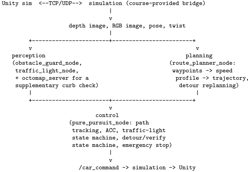
Figure 1: High-level node/data-flow architecture. Perception and planning consume the simulator’s sensor/pose streams independently and run in parallel; control is the only node that combines their outputs and the sole path to /car_command — no other node talks to the simulator directly.
