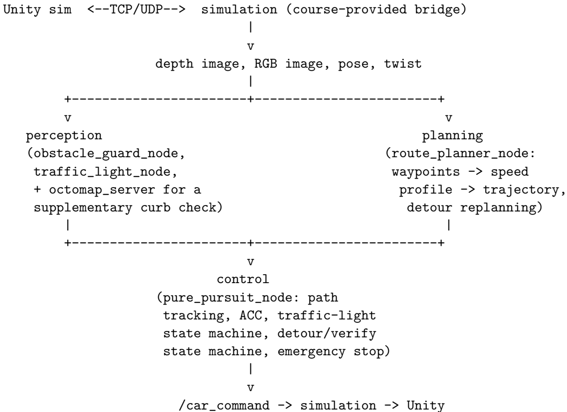
Figure 1: High-level node/data-flow architecture. Perception and planning consume the simulator’s sensor/pose streams independently and run in parallel; control is the only node that combines their outputs and the sole path to /car_command — no other node talks to the simulator directly.
