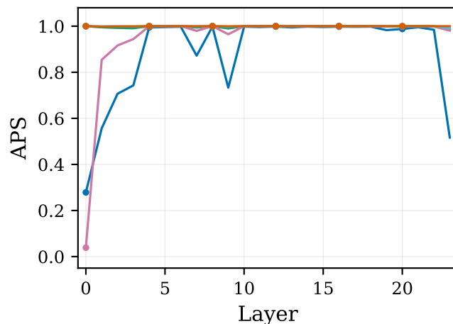
Greater-Than: Activation Preservation Score (APS)
