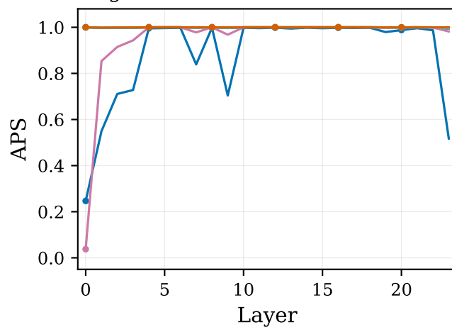
Docstring: Activation Preservation Score (APS)
