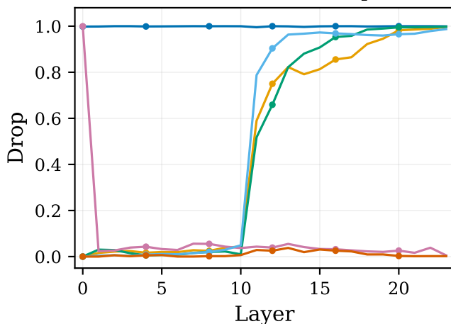
Greater-Than: Behavioral Drop
