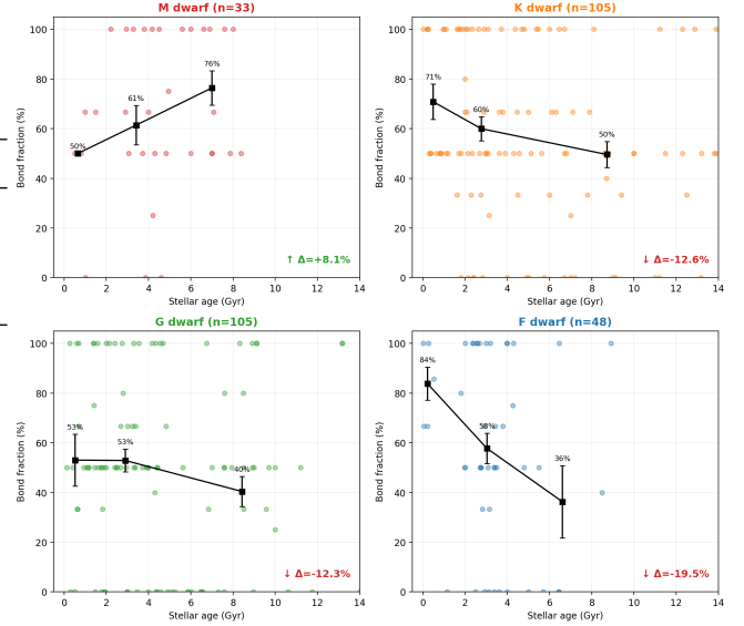
Bond Fraction vs. Stellar Age — M dwarfs build bonds, others decay
