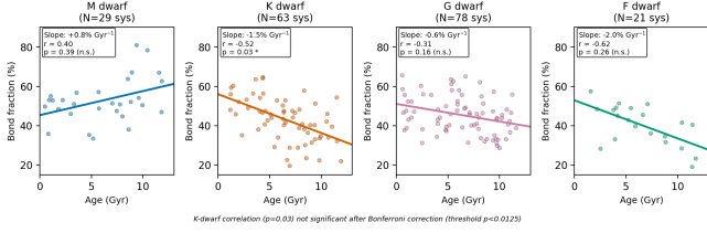
Figure 4. System-level bond fraction as a function of isochronal age, by stellar type. The U-shape in bond fraction across mass is mirrored by opposite age correlations: M dwarfs show tentatively increasing bond fraction with age ( +0.8\% \text{ Gyr}^{-1} , or approximately +8\% over 10 Gyr); K, G, and F dwarfs all show decreasing bond fraction with age.
