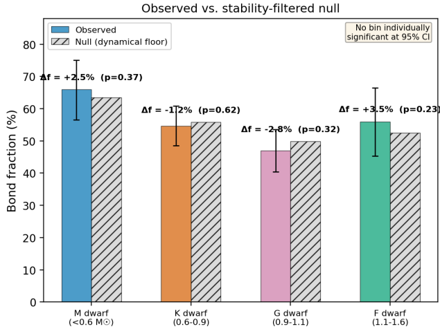
Figure 3. Observed bond fraction (system-level mean \pm 95% bootstrap CI) compared to the stability-filtered null. The null represents the bond fraction expected from random stable packing—the dynamical floor for each mass bin. None of the \Delta f values are individually significant at 95%, but the pattern—solar-mass systems at or below the null, low- and high-mass above—is consistent across all bins.
