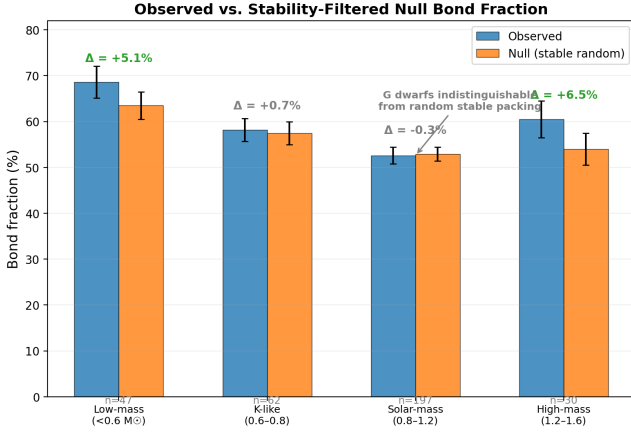
Figure 3. Observed bond fraction compared to a stability-filtered null ensemble. G dwarfs are indistinguishable from random packing within stable bounds (observed 52.6% vs. null 52.9%), while M and F dwarfs show genuine excess bonding.
