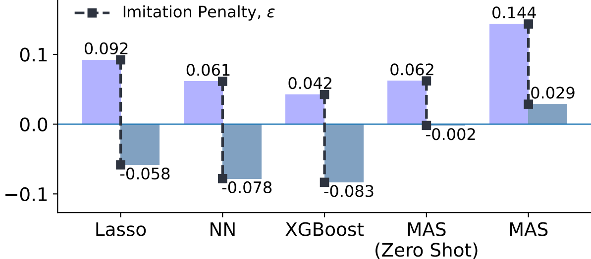
Average Net Return (Test Set)
