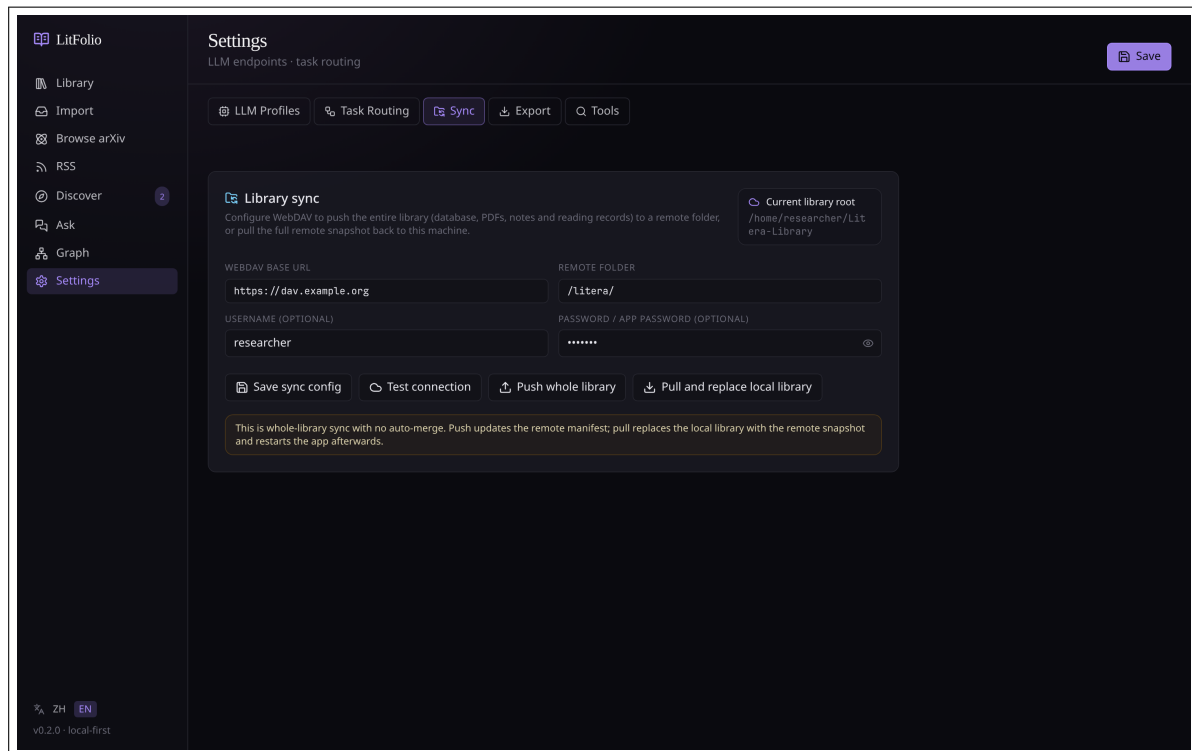
Figure 15.2 WebDAV Sync panel. After configuring the URL and credentials, you can Push (local→remote) or Pull and Replace Local (remote→local, which first backs up the local state to backups/sync/ ).
