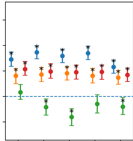
FooTweets
