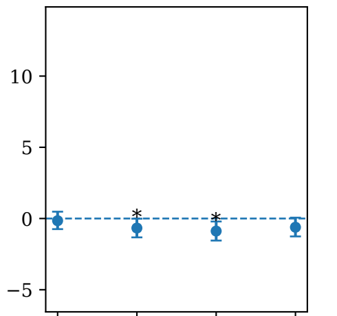
RoCS-MT
