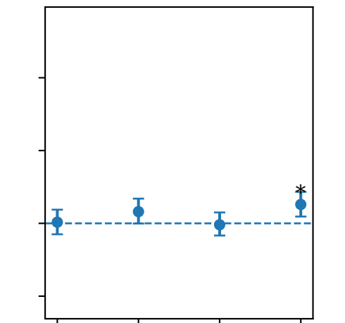
FooTweets
