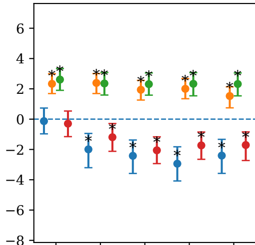
RoCS-MT
