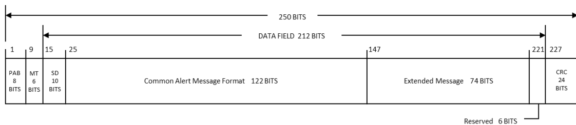
Figure 4.2-1 MT44 Format
