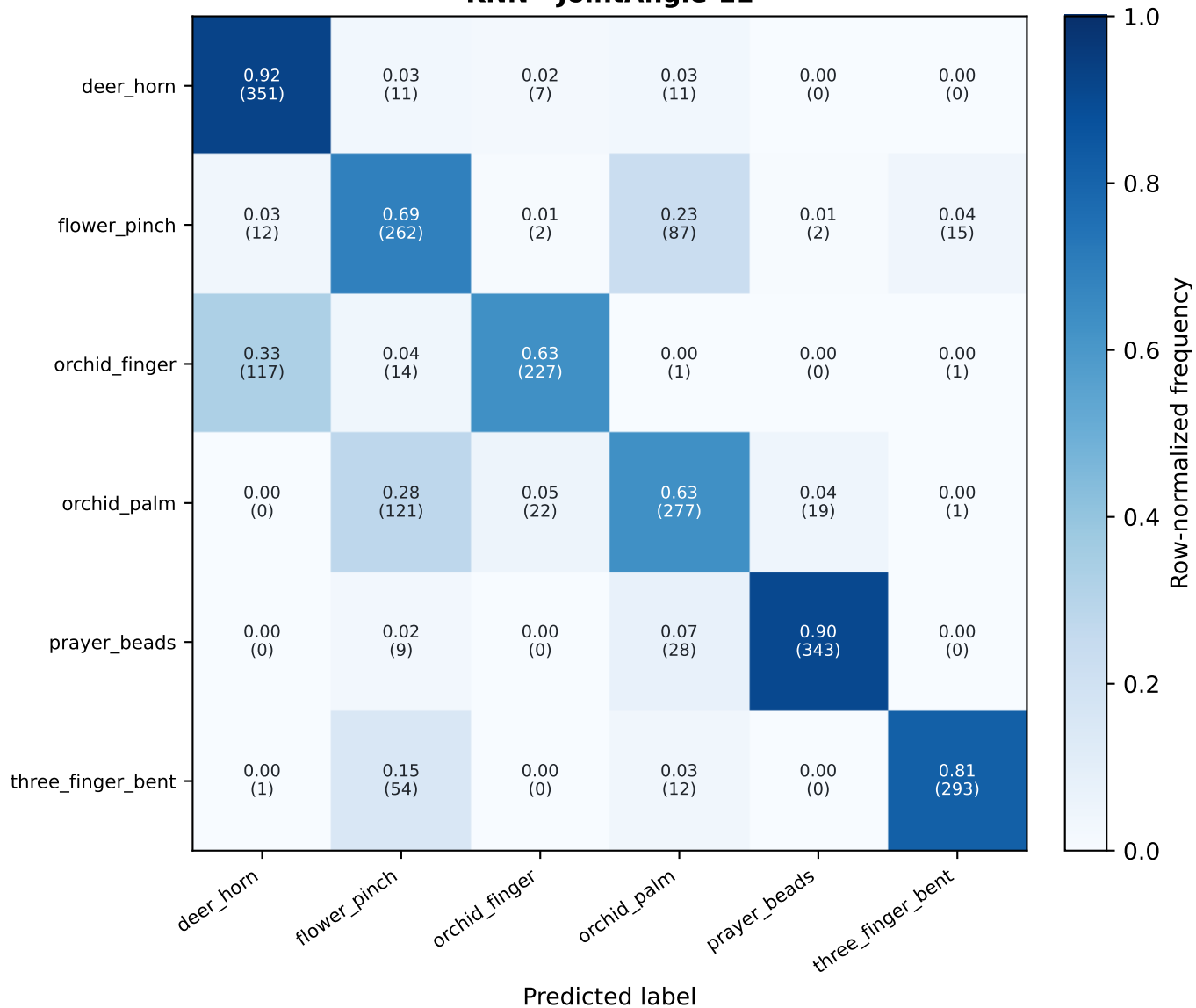
KNN - JointAngle-11
