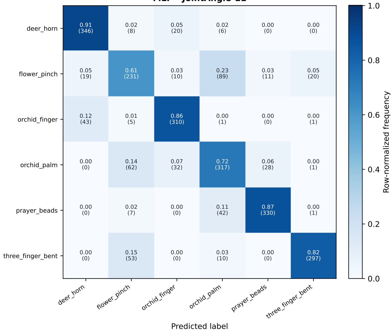
MLP - JointAngle-11
