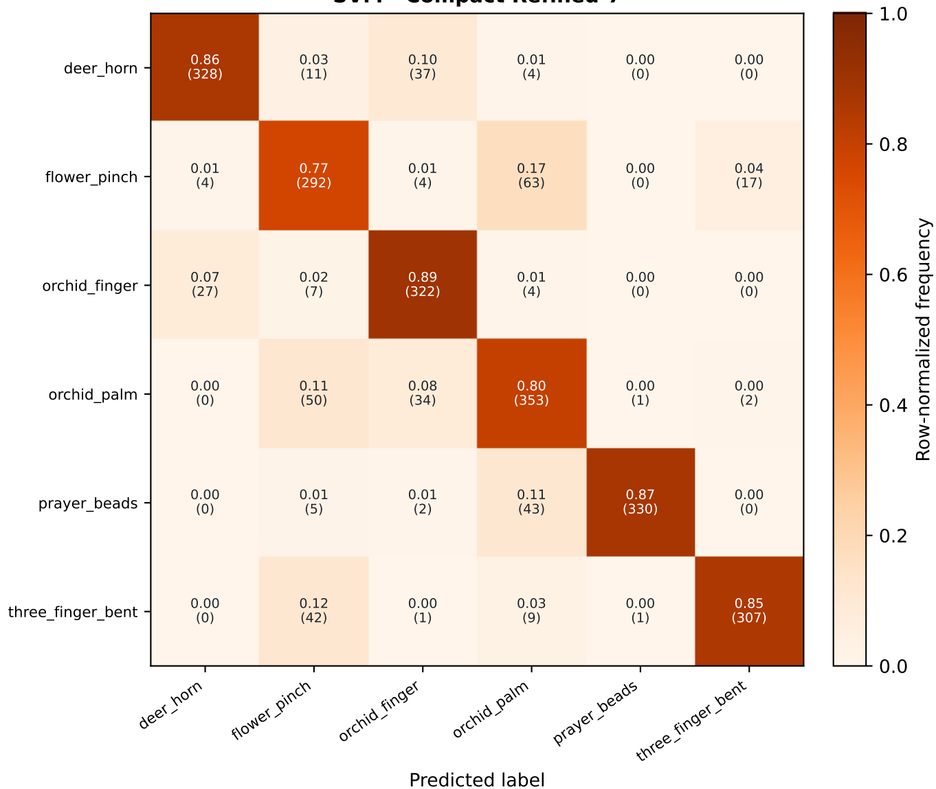
SVM - Compact Refined-7
