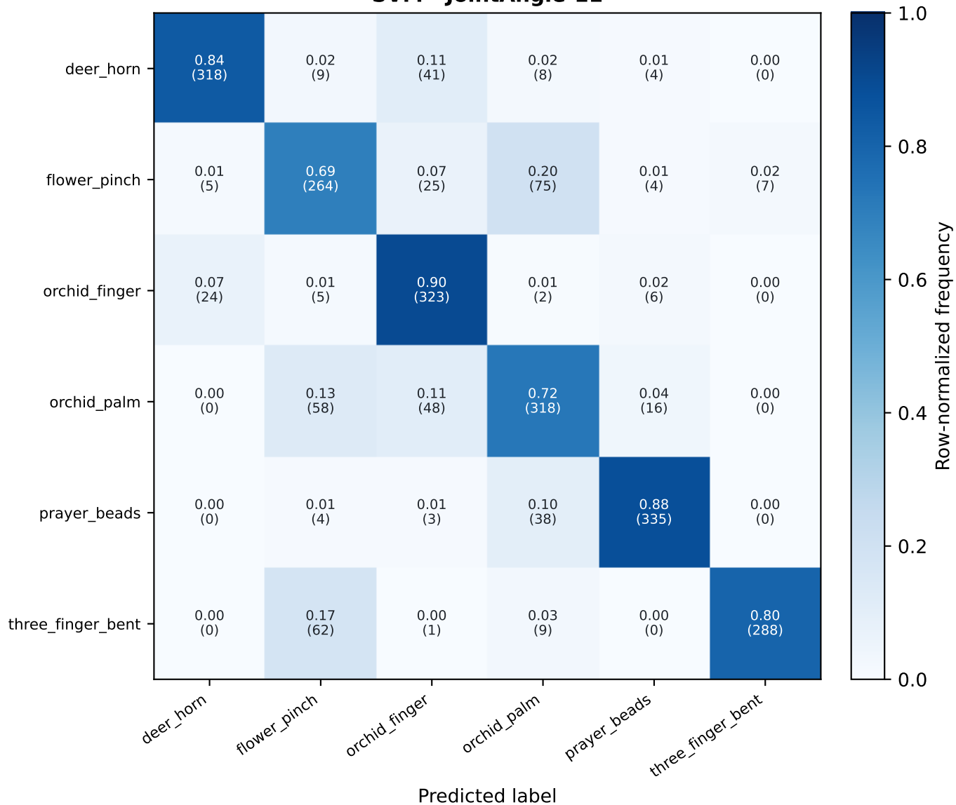
SVM - JointAngle-11
