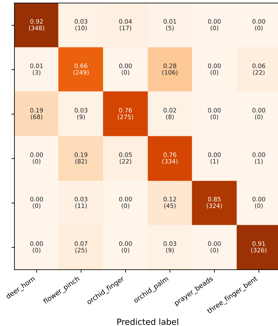
KNN - Compact Refined-7
