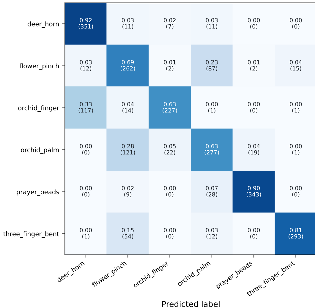
KNN - JointAngle-11
