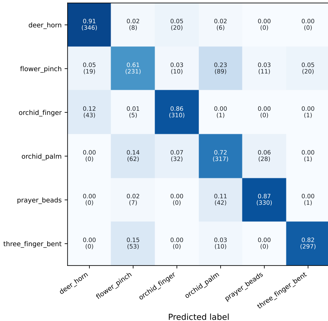
MLP - JointAngle-11
