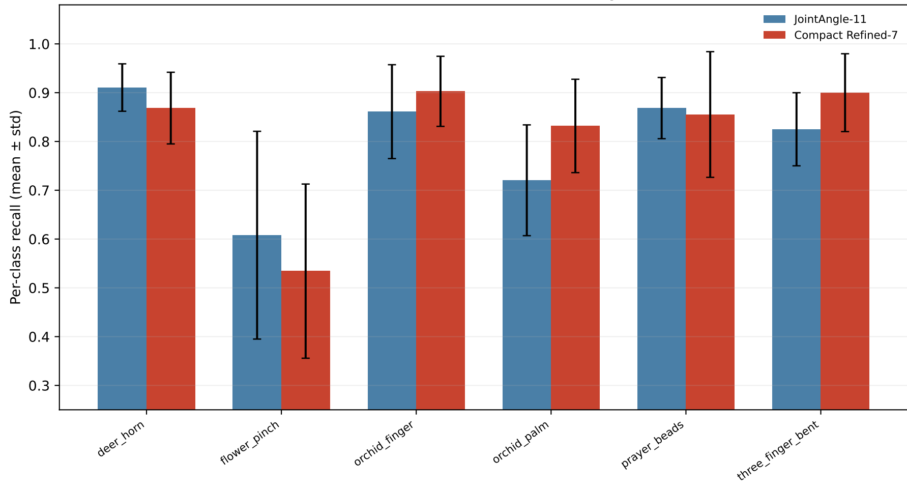
MLP Per-class Recall Stability
