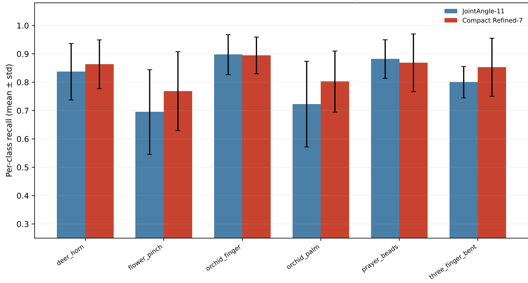
SVM Per-class Recall Stability
