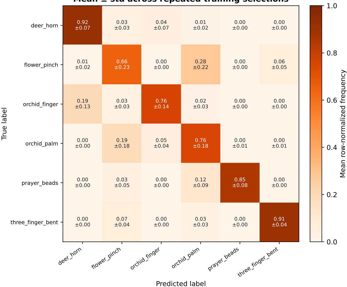
KNN - Compact Refined-7 Mean \pm std across repeated training selections
