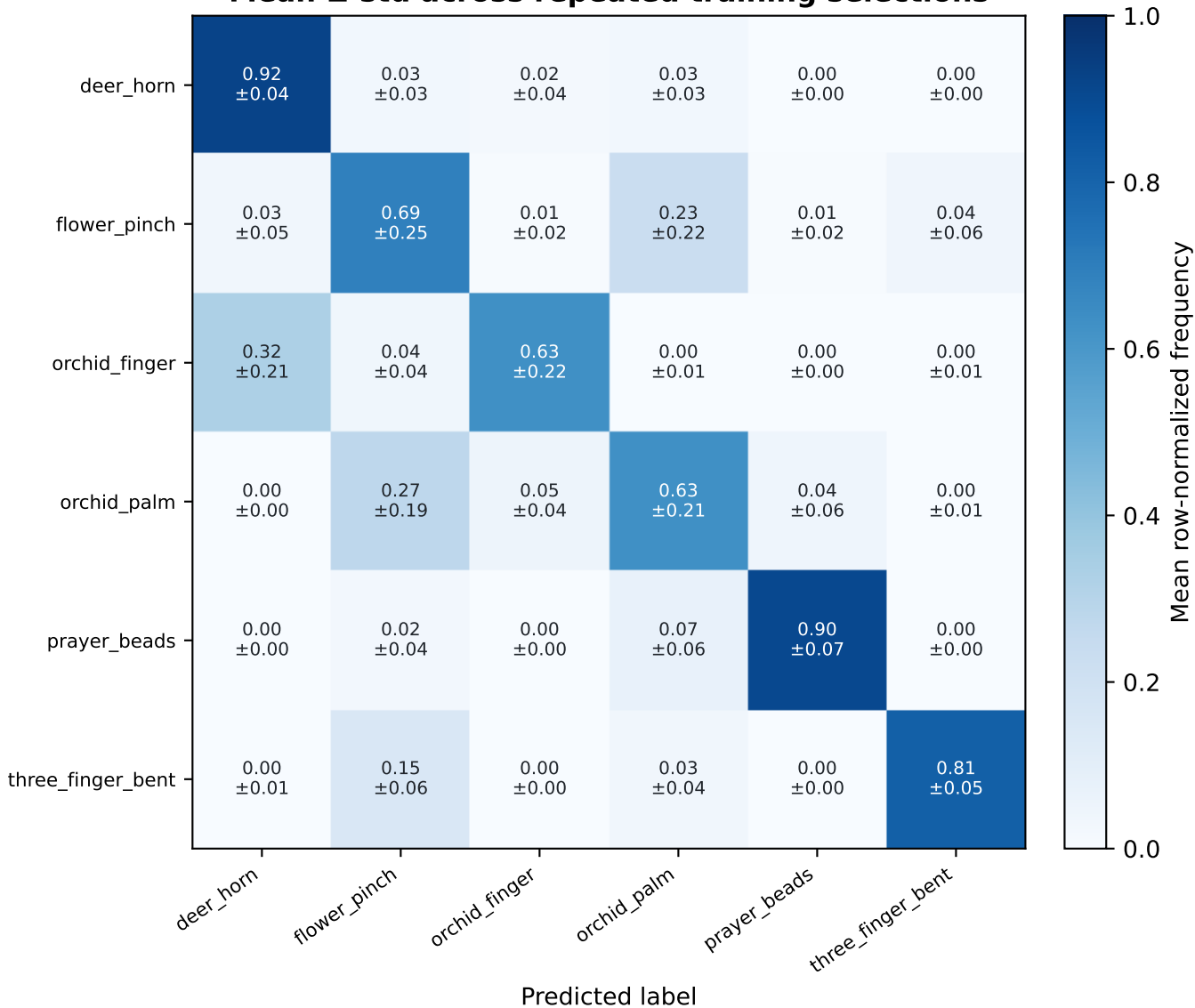
KNN - JointAngle-11 Mean \pm std across repeated training selections
