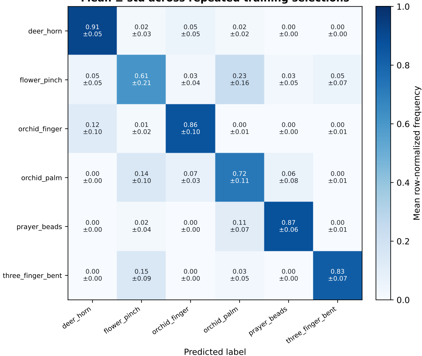
MLP - JointAngle-11 Mean \pm std across repeated training selections
