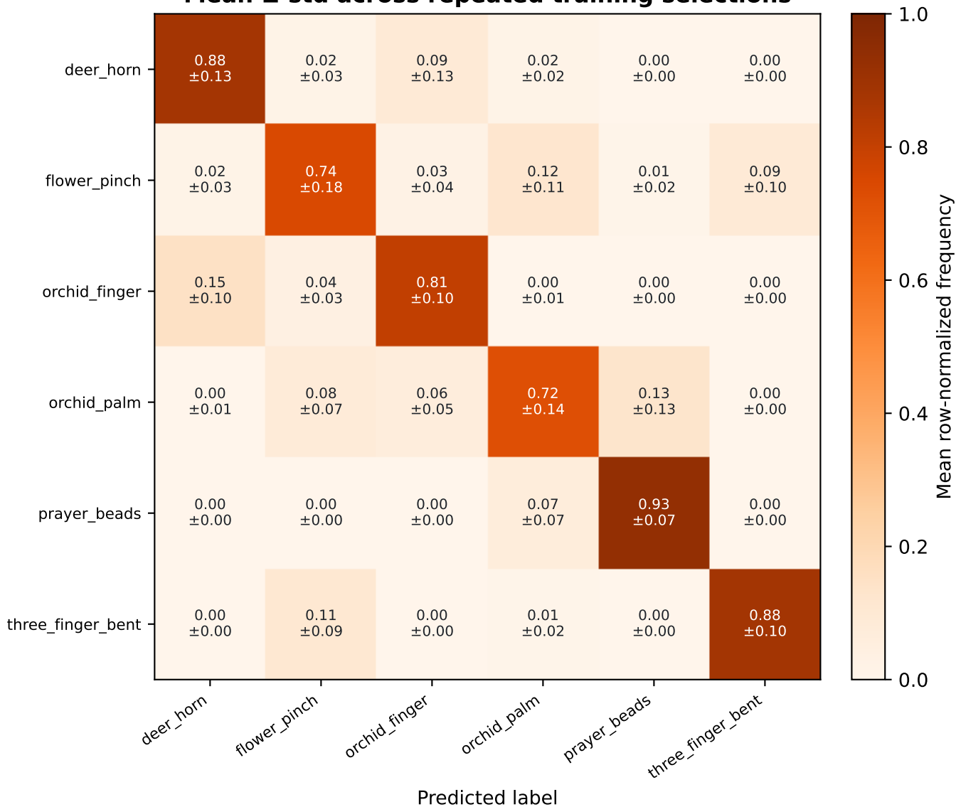
RandomForest - Compact Refined-7 Mean \pm std across repeated training selections
