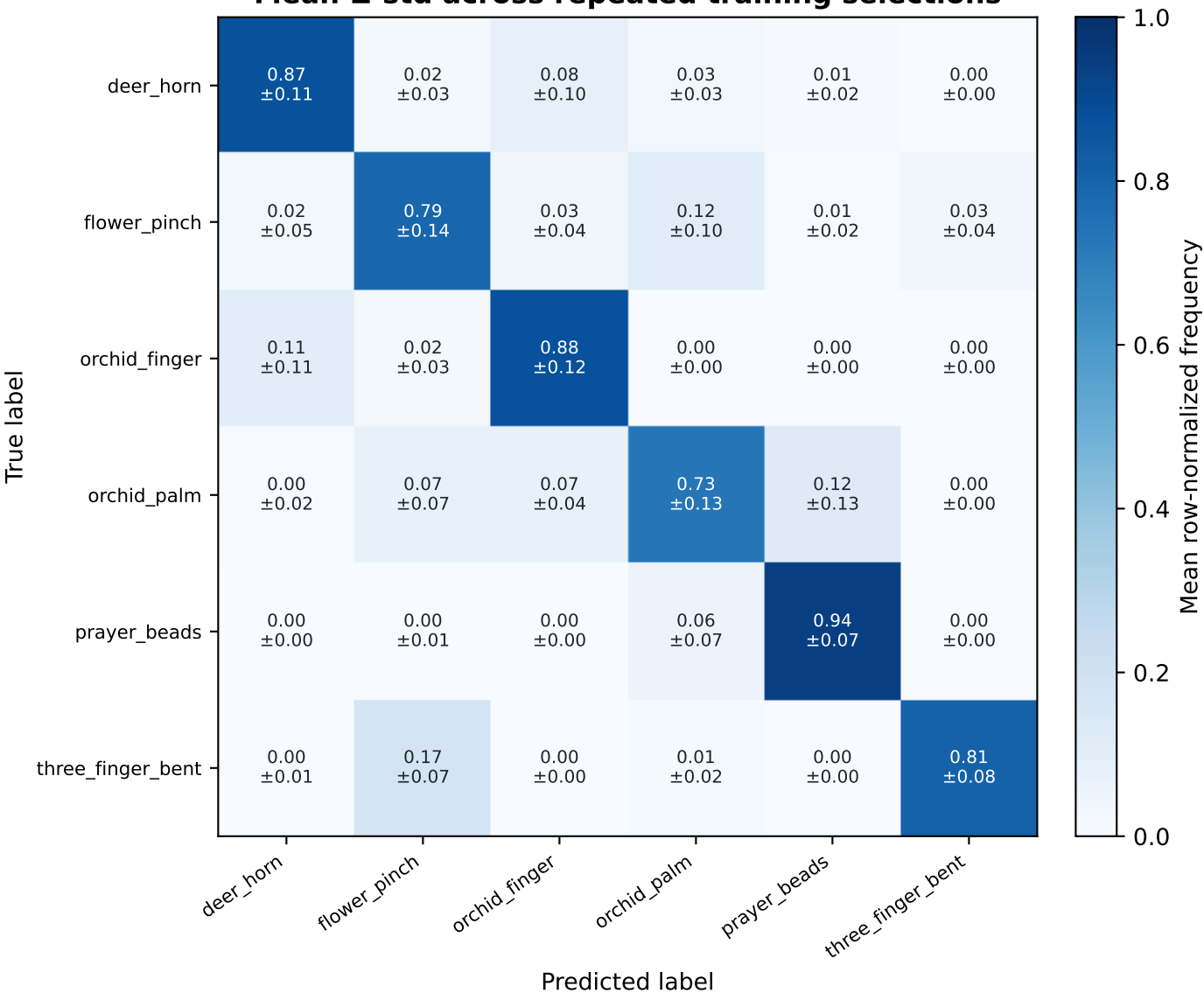
RandomForest - JointAngle-11 Mean \pm std across repeated training selections
