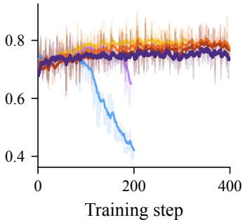
Training reward
