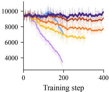
Response length (tokens)
