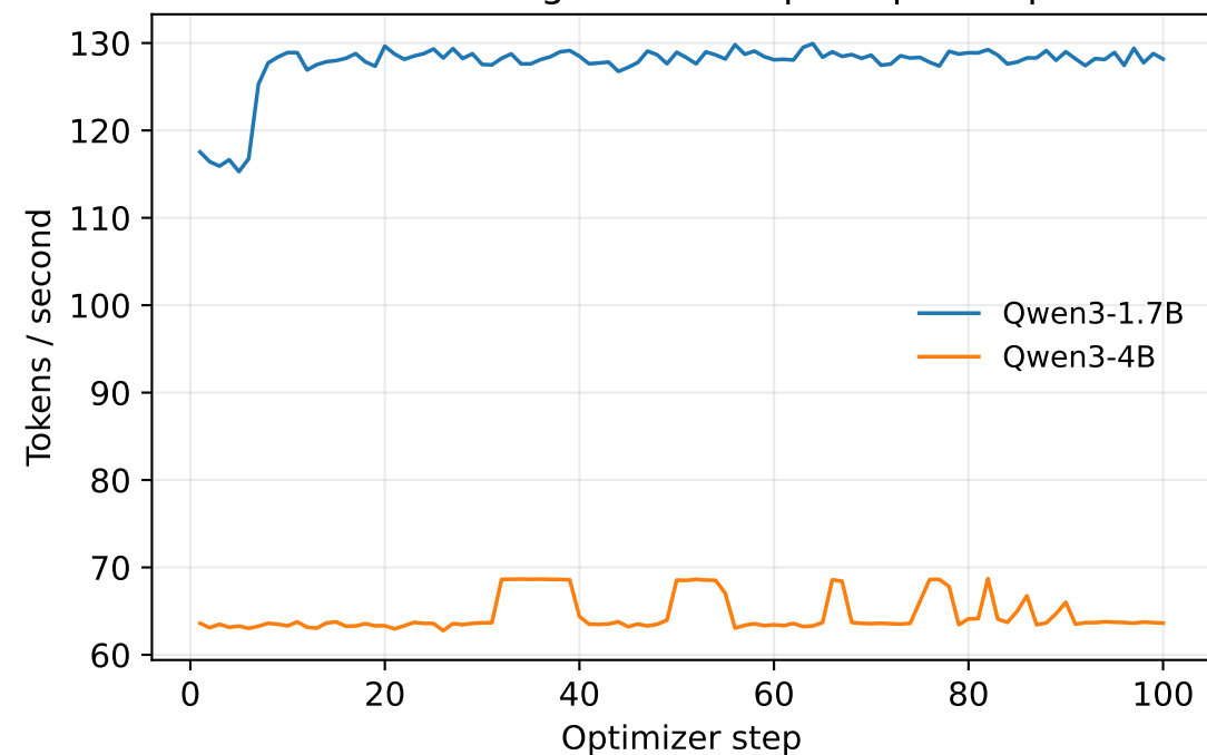
Mean vLLM generation speed per step
